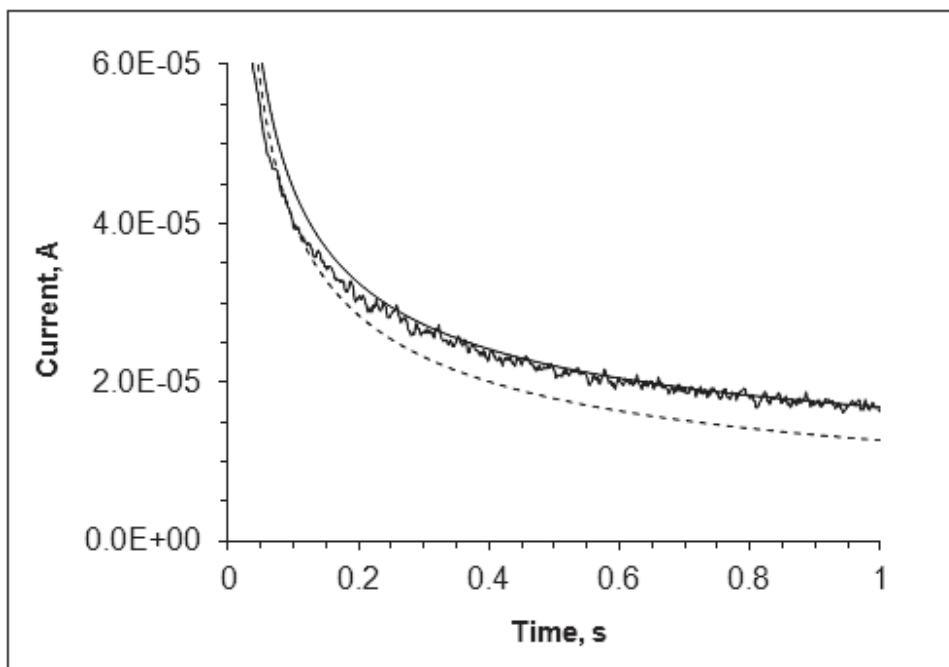
Figure 4. Experimental chronoamperogram for the Au micro-electrode array in 1.0 mM \text{FeCO}_2\text{H} upon potential step from 0.0 to 0.5 V vs. Ag/AgCl (continuous, noisy trace). Calculated Cottrellian (dashed line) and Shoup-Szabo (continuous line) current transients for 190 disks of r = 125 \mu\text{m} each.
